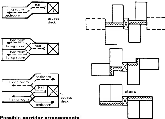
② Possible corridor arrangements
